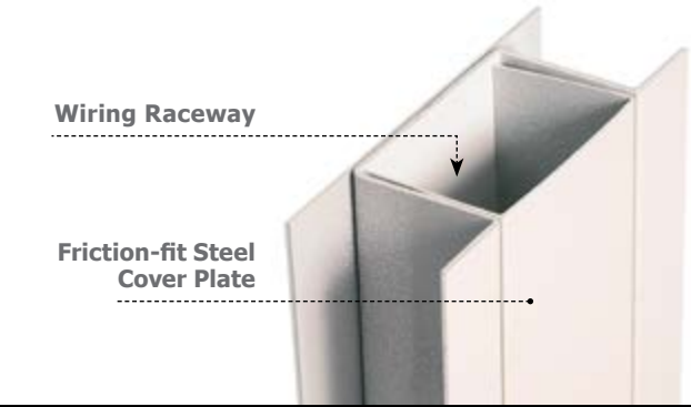
1.75 inch, Load-Bearing Steel Wiring Stud - 16 gauge
